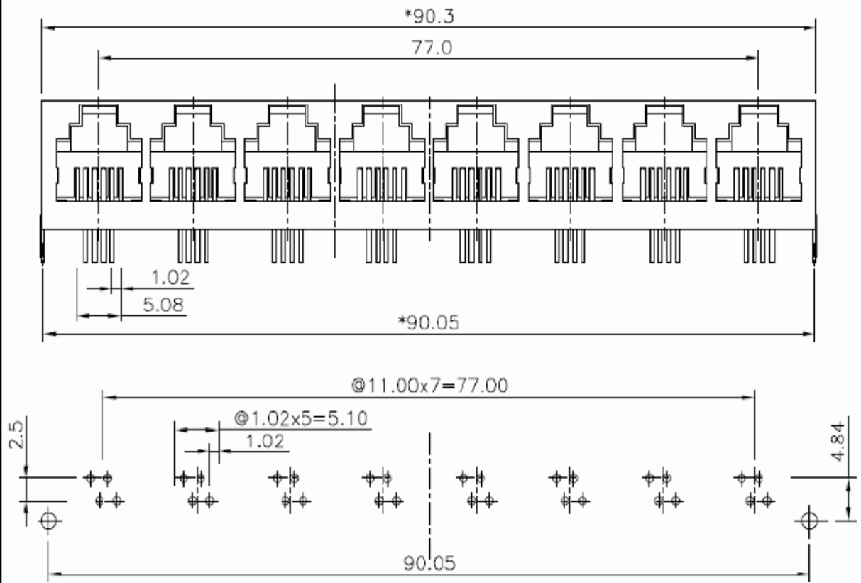
PC Board Layout Component Side Shown
